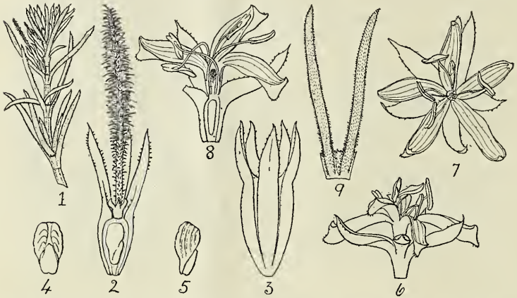
FIG. 2. Carpacoe vaginellata , Salter. 1. Portion of female plant (natural size). 2. Longitudinal section through female flower \times 4 . 3. Fruit \times 4 . 4 and 5. Inner portion of the fruit (containing the seed) with the outer ribbed portion removed and showing the tubercle \times 4 . 6. Hermaphrodite flower, side view \times 4 . 7. Hermaphrodite flower, front view \times 4 . 8. Longitudinal section through hermaphrodite flower \times 4 . 9. Pair of leaves \times 2 . (Salter 6271.) Del. W. F. Barker.
